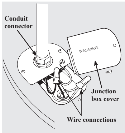
Water heater junction box
