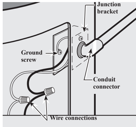
Point-of Use water heater junction bracket.
